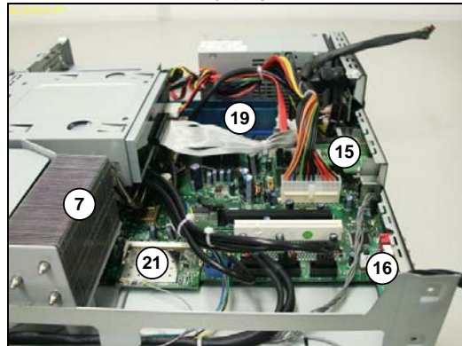
Right View
