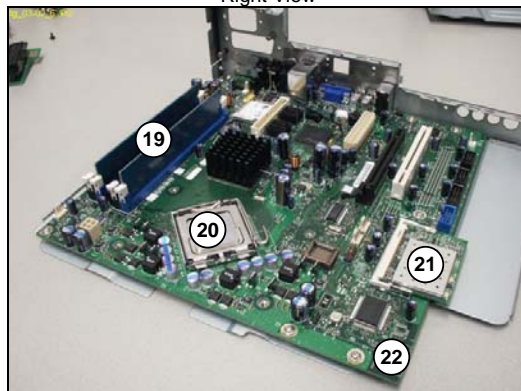
Motherboard subassembly
