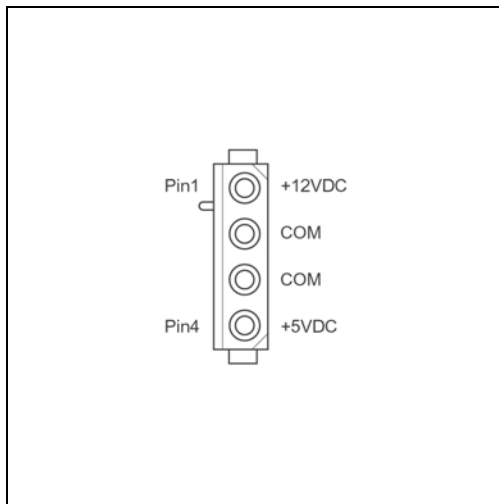
Peripheral Power Connector, 4-pin
