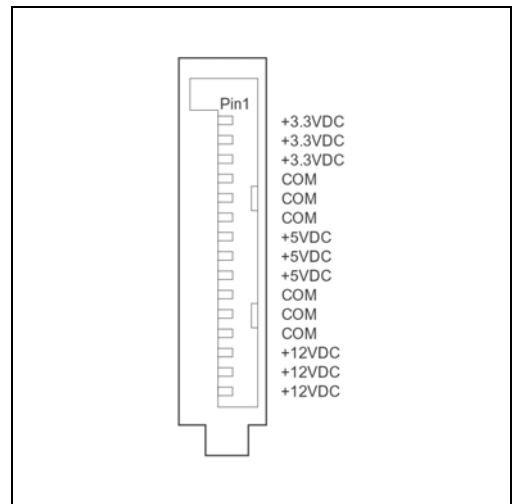
Serial ATA (SATA) Power Connector
