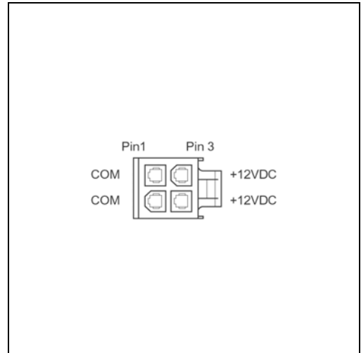
+12V Power Connector, 2x2-pin
