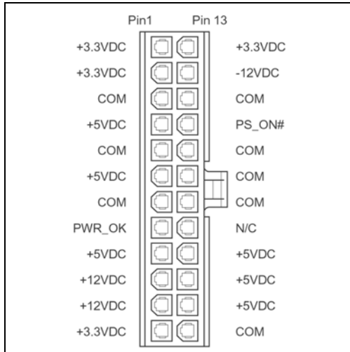
Main Power Connector, 2x12-pin
